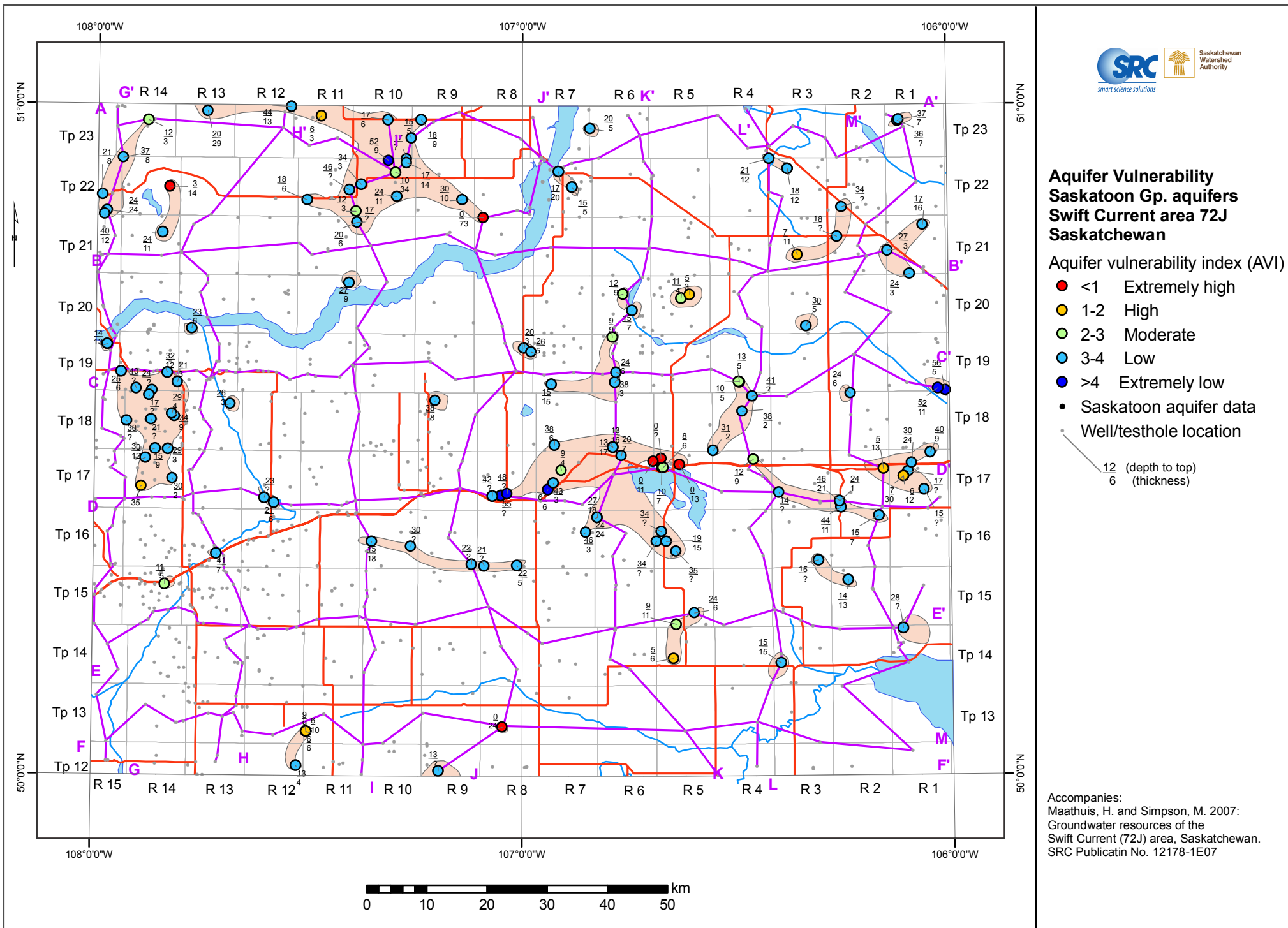
Aquifer vulnerability index (AVI) of the Saskatoon Group aquifers in the Swift Current area
