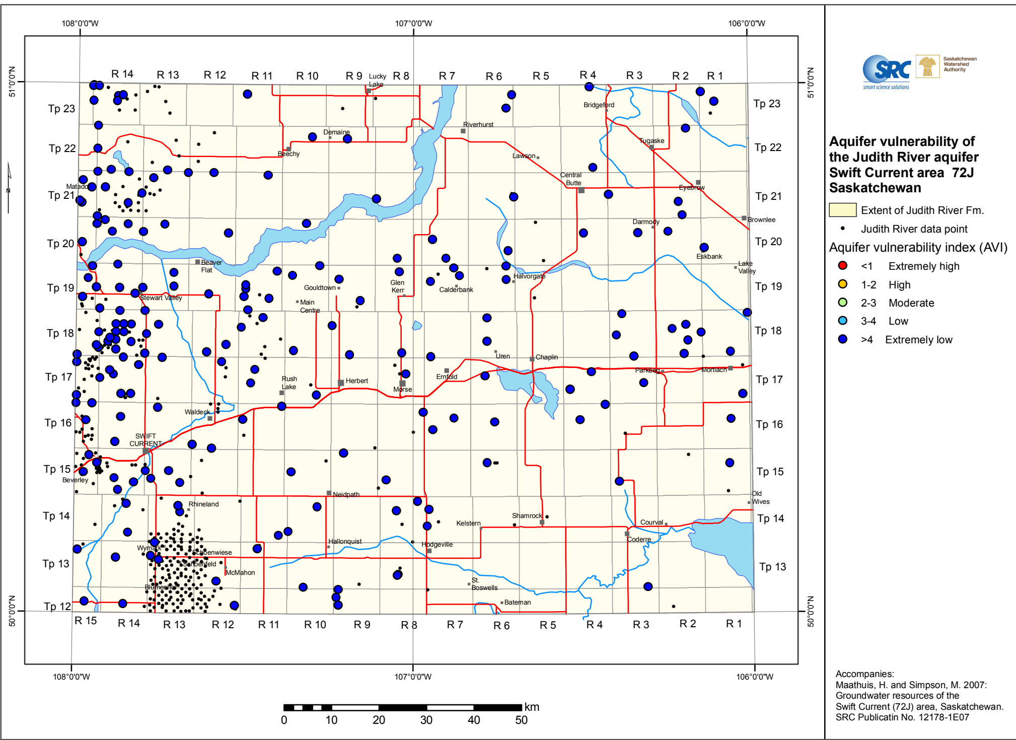
Aquifer vulnerability index (AVI) of the Judith River aquifer in the Swift Current area
