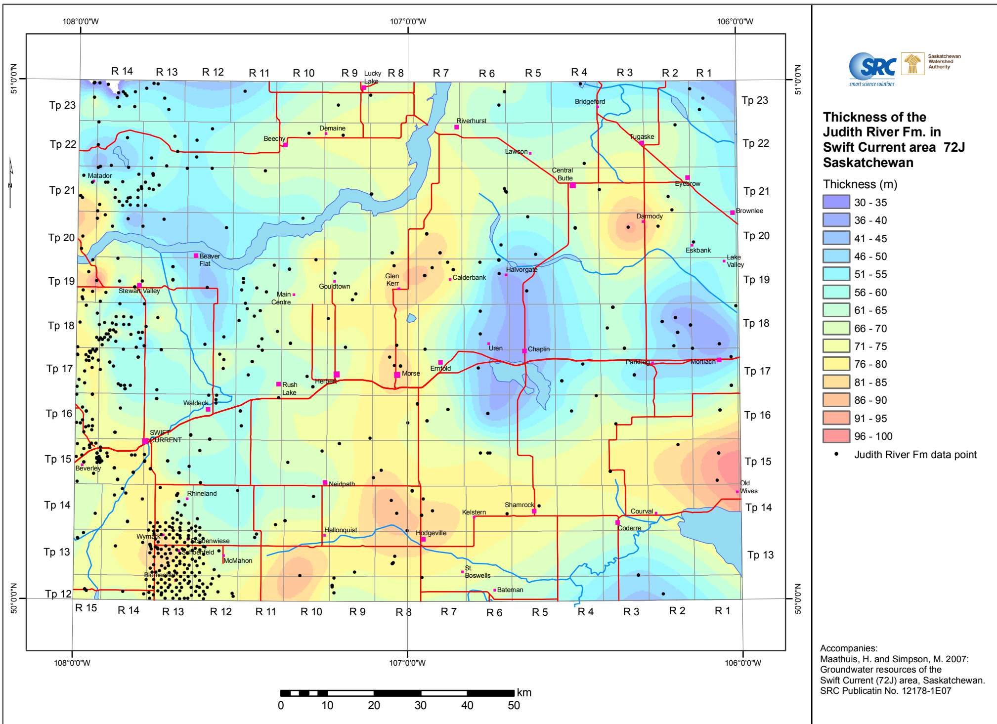
Thickness of the Judith River Formation in the Swift Current area
